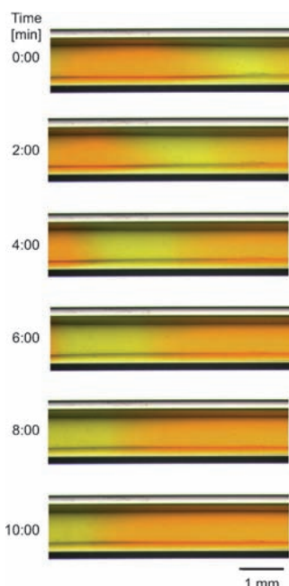
Figure 2. Time-course images of the peristaltic motion of the tubular poly(NIPAAm- co -Ru(bpy) 3 ) gel adhering to the inner wall of a glass capillary. Light green band moves from right to left, indicating thickening of the side walls.
