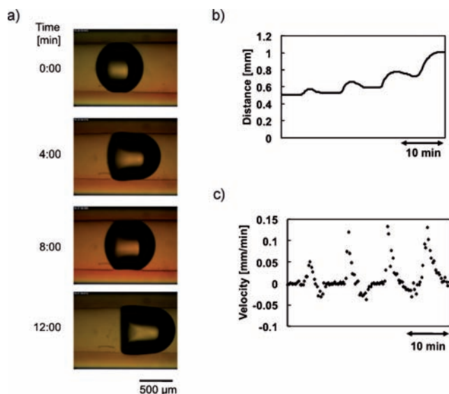
Figure 6. a) The autonomous transport of a \text{CO}_2 bubble in the gel tube by peristaltic pumping. b) Change in the position of the bubble. c) The velocity of the bubble.
