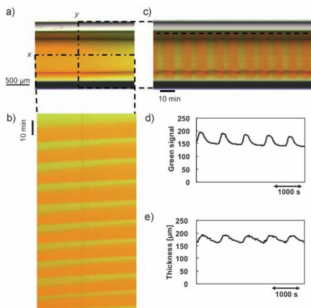
Figure 3. Time-series image analysis of the peristaltic motion of the tubular poly(NIPAAm- co -Ru(bpy) 3 ) gel shown in Figure 2. a) One frame image extracted from the movie. b) Spatiotemporal pattern constructed by lining up the dashed x line time sequentially. c) Spatiotemporal pattern constructed by lining up the dashed y line time sequentially. d) Redox changes at a fixed point in the gel layer, which is expressed as an intensity of the green signal along the dashed line in (c). e) Change in thickness of the gel layer at a fixed point, which is derived from (c).
